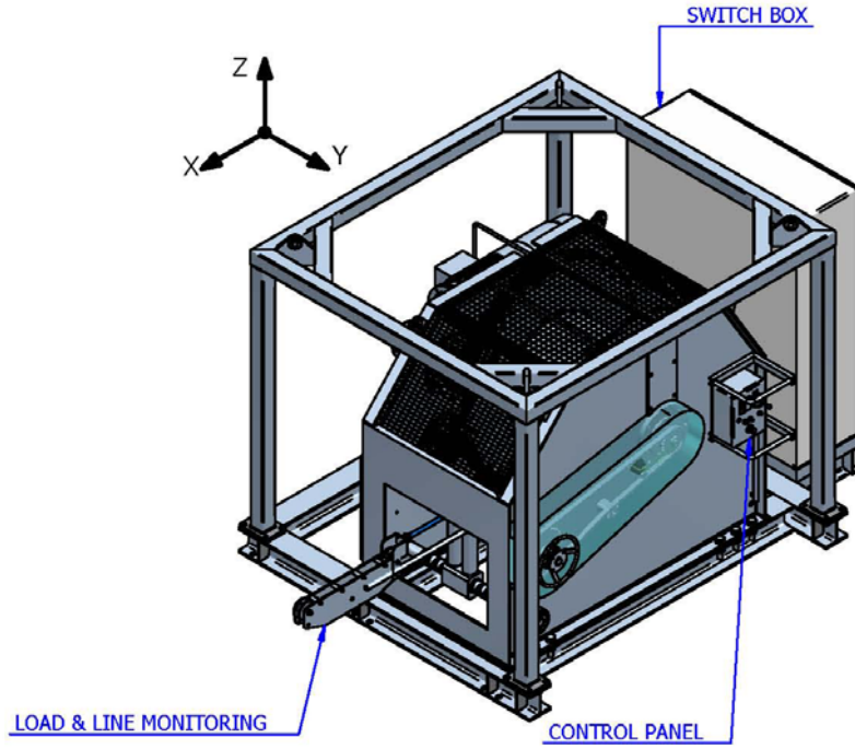
Abandon & Recovery (A&R) Winches
