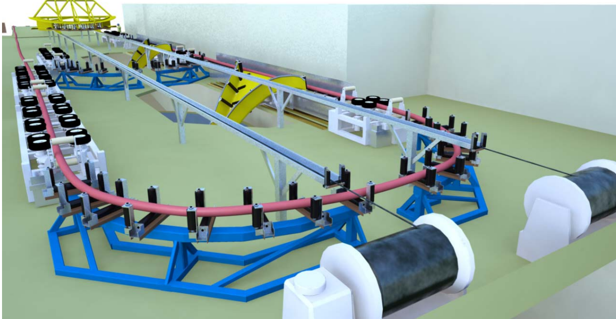
Arrangement on Cable Handling Deck with Cable Deployment Bow
