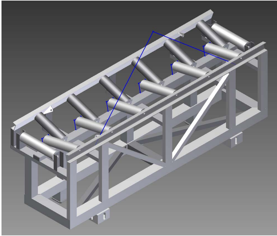
Cable Support Roller Sections
