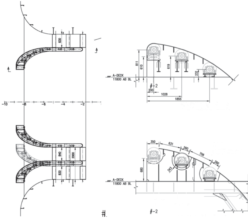
Cable Stern Chutes
